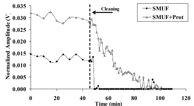
Figure 3: Cleaning of SMUF and SMUF with whey protein (SMUF+Prot) deposition curves assessed with the MSS
