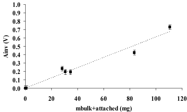
Figure 4: Relation between the A_{inv} and the mass of shampoo that remains in the flow cell ( m_{bulk+attached} ) after the cleaning procedure ( R^2=0.9633 )
