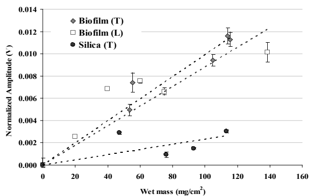
Figure 2: Variation of the MSS normalized amplitude with the wet mass per unit of area: Pseudomonas fluorescens biofilm under turbulent flow (♦), Pseudomonas fluorescens biofilm under laminar flow (□) and silica deposit under turbulent flow (●)
